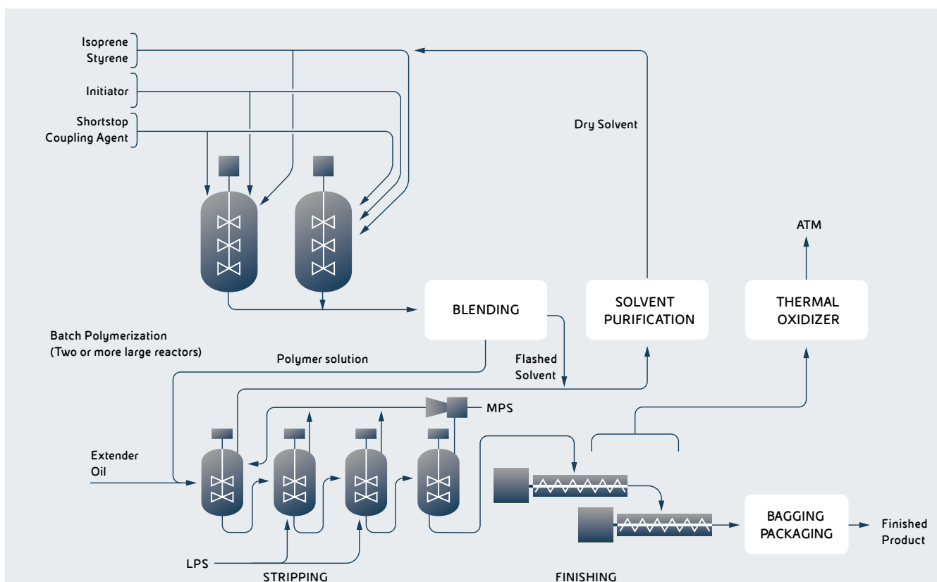
SIS • process scheme
